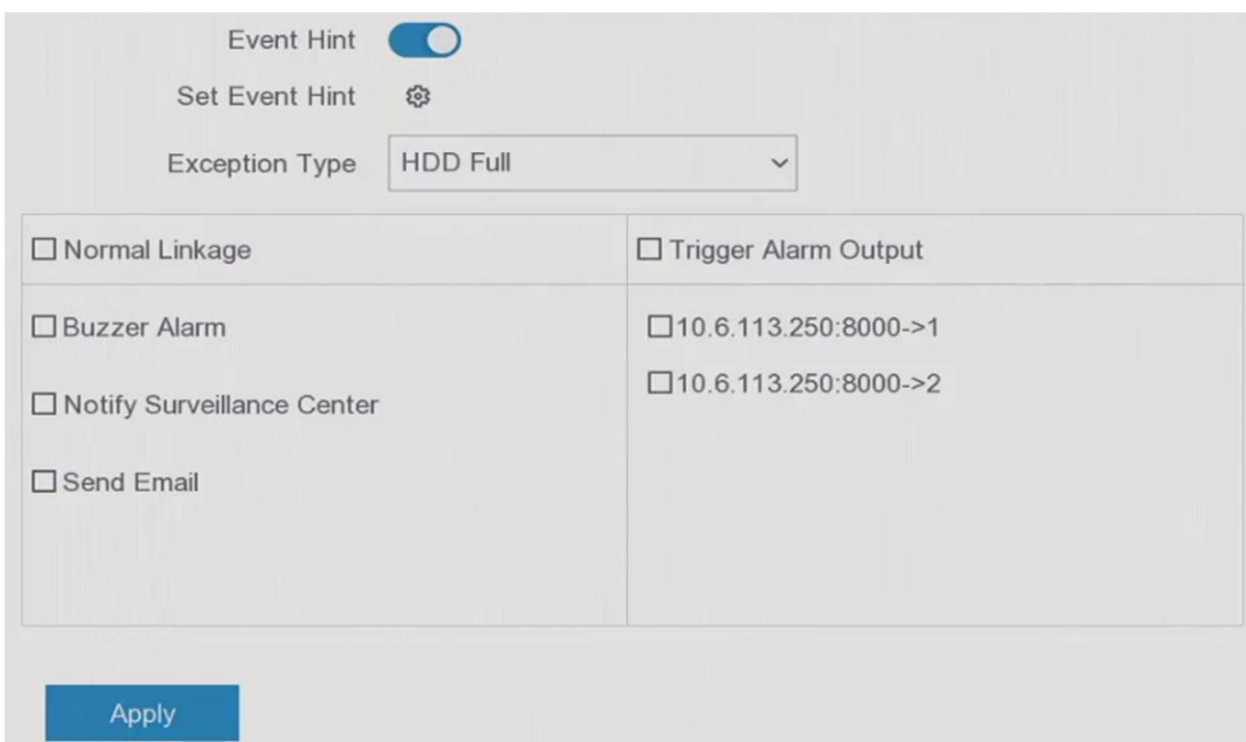
Figure 6-19 Exceptions
